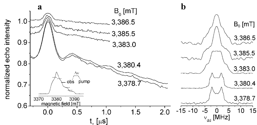
Figure 4. W-band DEER results (40 K) of doubly nitroxide-labeled \tau_{C14} ( \sim 60 \mu\text{M} ). (a) DEER raw data measured at 40 K at different magnetic fields. The inset shows the field sweep echo-detected EPR spectrum of this sample at 40 K, indicating the positions of the pump and observe pulses. Experimental conditions are as in Figure 2. The measurement time was 0.5 h for the field of maximum EPR signal and 13 h at the highest field. (b) Fourier transform of the time domain DEER data obtained after subtraction of the background.
