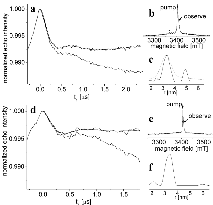
Figure 5. W-band DEER results (25 K) for \tau_{C14} doubly labeled with \text{Gd}^{3+} -4MMDPA and \text{Gd}^{3+} -3MDPA ( \sim 100 \mu\text{M} ). (a) Raw DEER time domain data of \tau_{C14} tagged with 4MMDPA- \text{Gd}^{3+} , DEER trace after subtraction of the background decay, and the corresponding superimposed calculated trace obtained with the distance distribution shown in (c). Measurement time \sim 8 h. The experimental conditions were the same as in Figure 3. (b) Echo-detected EPR spectrum of \tau_{C14} tagged with 4MMDPA- \text{Gd}^{3+} , recorded with the two-pulse echo sequence. Arrows mark the positions of the pump and observe pulses. (c) \text{Gd}^{3+} - \text{Gd}^{3+} distance distribution. The dashed curve was obtained by a Gaussian fit. The calculated DEER trace in (a) was obtained with the Gaussian fit, and the same quality fit was obtained with the Tikhonov regularization. (d–f) Same as (a–c) except that \tau_{C14} was tagged with 3MDPA- \text{Gd}^{3+} .
